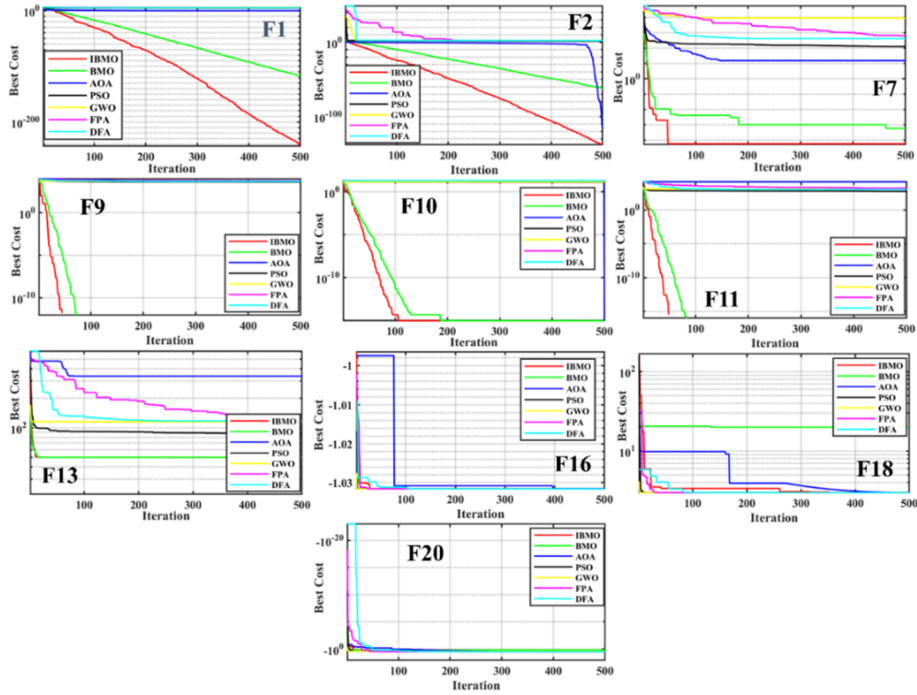
Fig. 3. Convergence Curves
